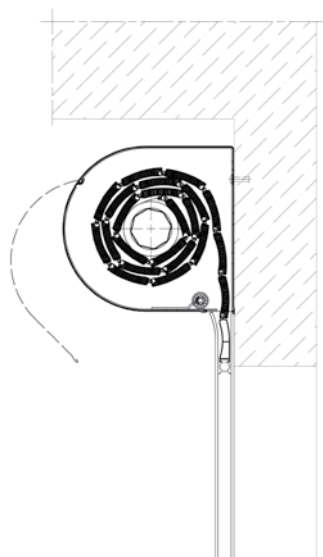
Tor - BGR/SKO-P
